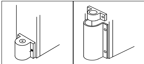
Combo Bottom Bearing/ Jamb Guard
